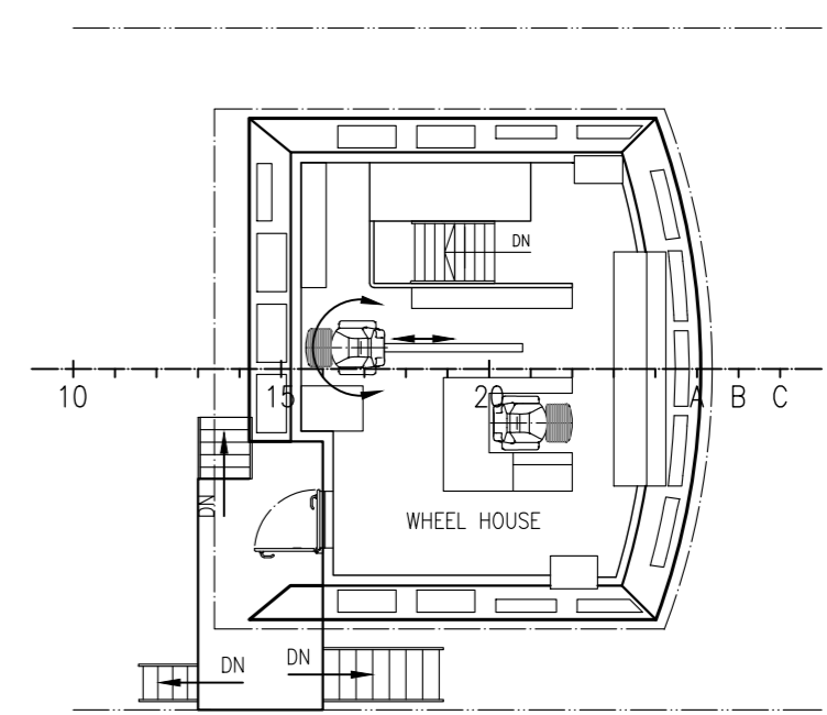
BRIDGE DECK
