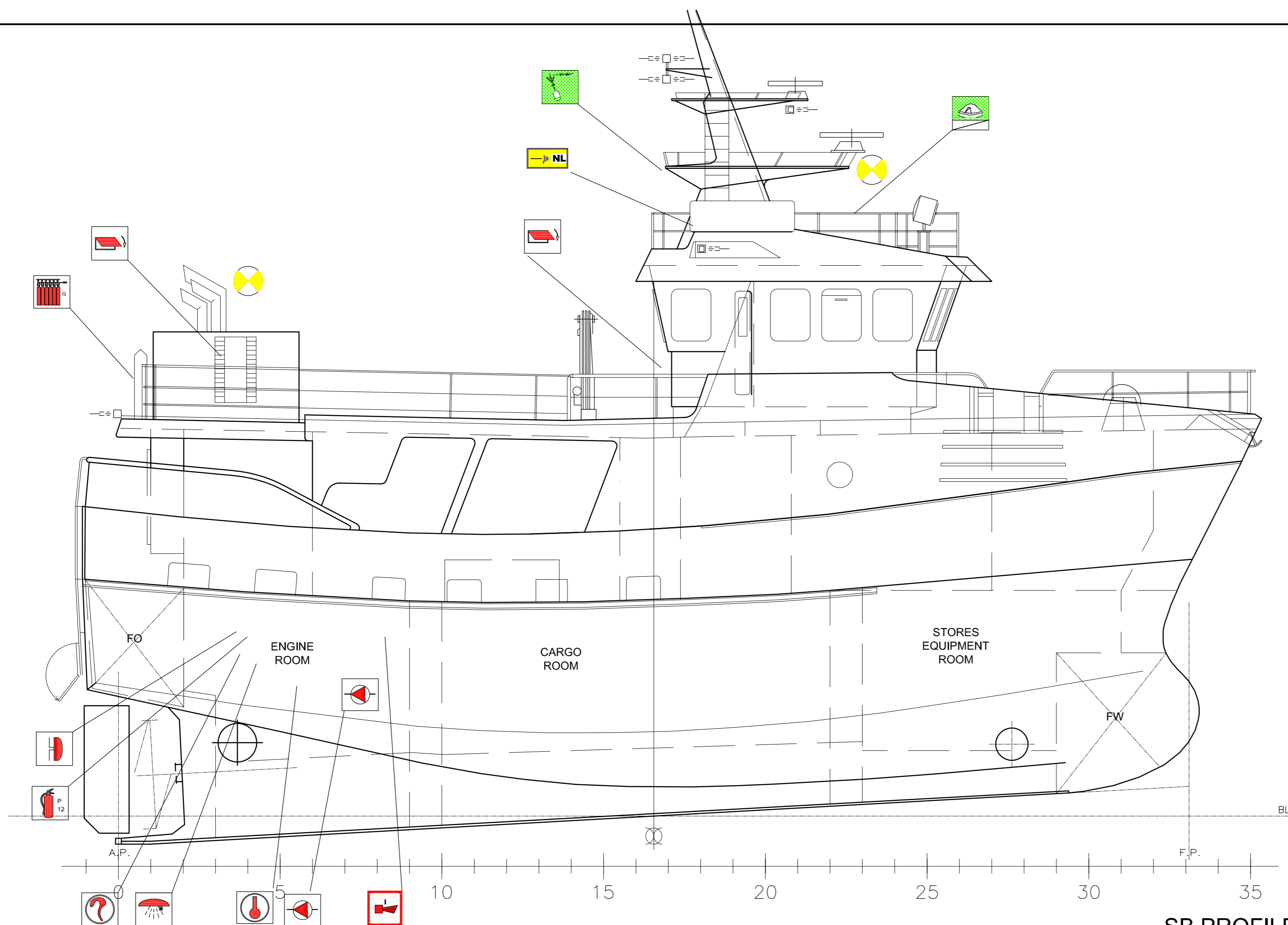
SB PROFILE
