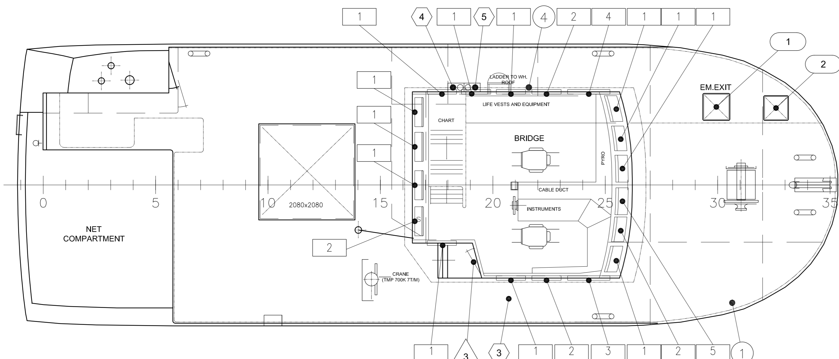
BOAT DECK/BRIDGE 6190
